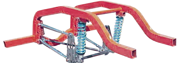
Picture shows deluxe 4-link frame package with 8 moly rod ends
